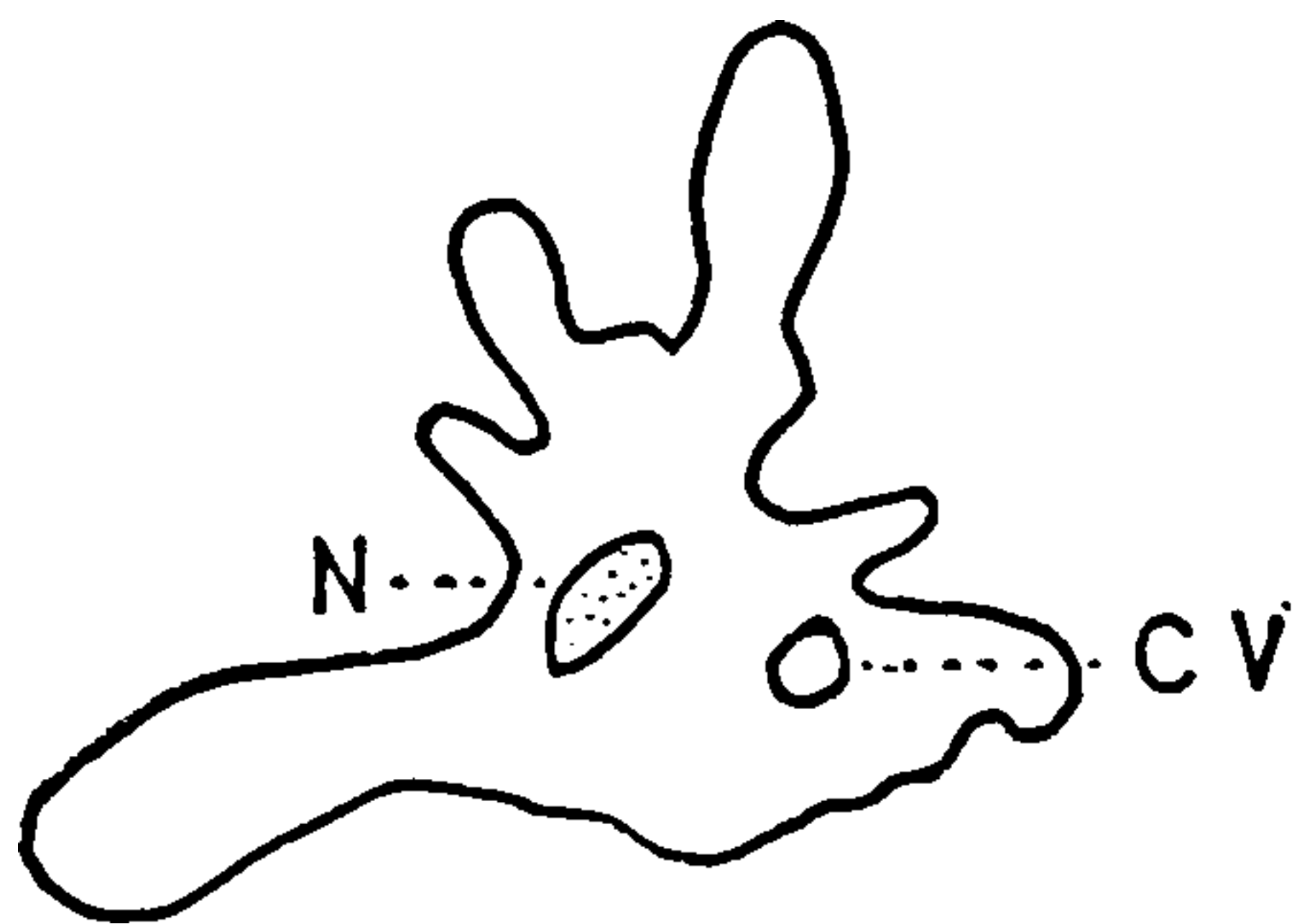
FIG. 1.—Diagram of an amoeba greatly magnified. The irregularly shaped mass of protoplasm is shown with N , its nucleus, and CV , a contractile vacuole, which expands and contracts.
